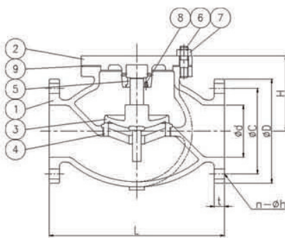
GLOBE VALVE
