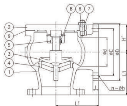
ANGLE VALVE
